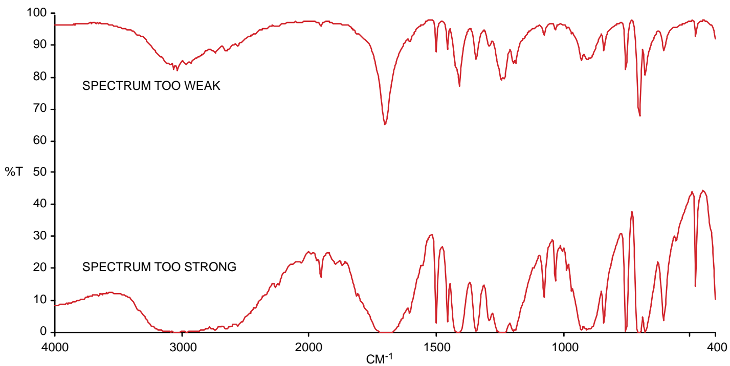
Figure 2 Phenyl Acetic Acid (i) Too Weak (ii) Too Strong
