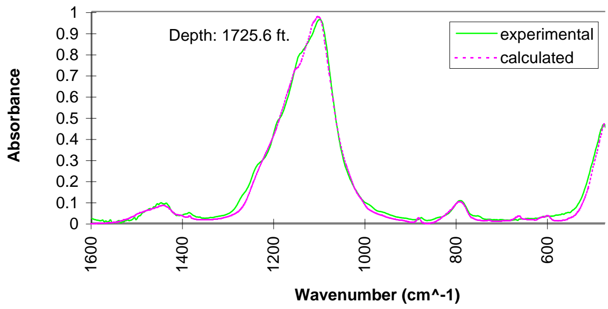
Figure 4. Comparison of experimental and calculated FTIR spectra McKittrick Fornt well #418, in the Cymric Field, Kern Country, CA, U
