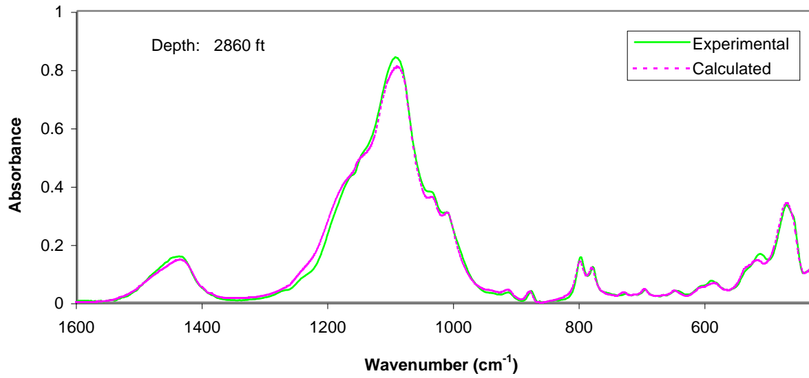
Figure 3. Comparison of experimental and calculated FTIR spectra for well KCL 44-375X, in the Pioneer Field, Kern Country, CA, USA.
