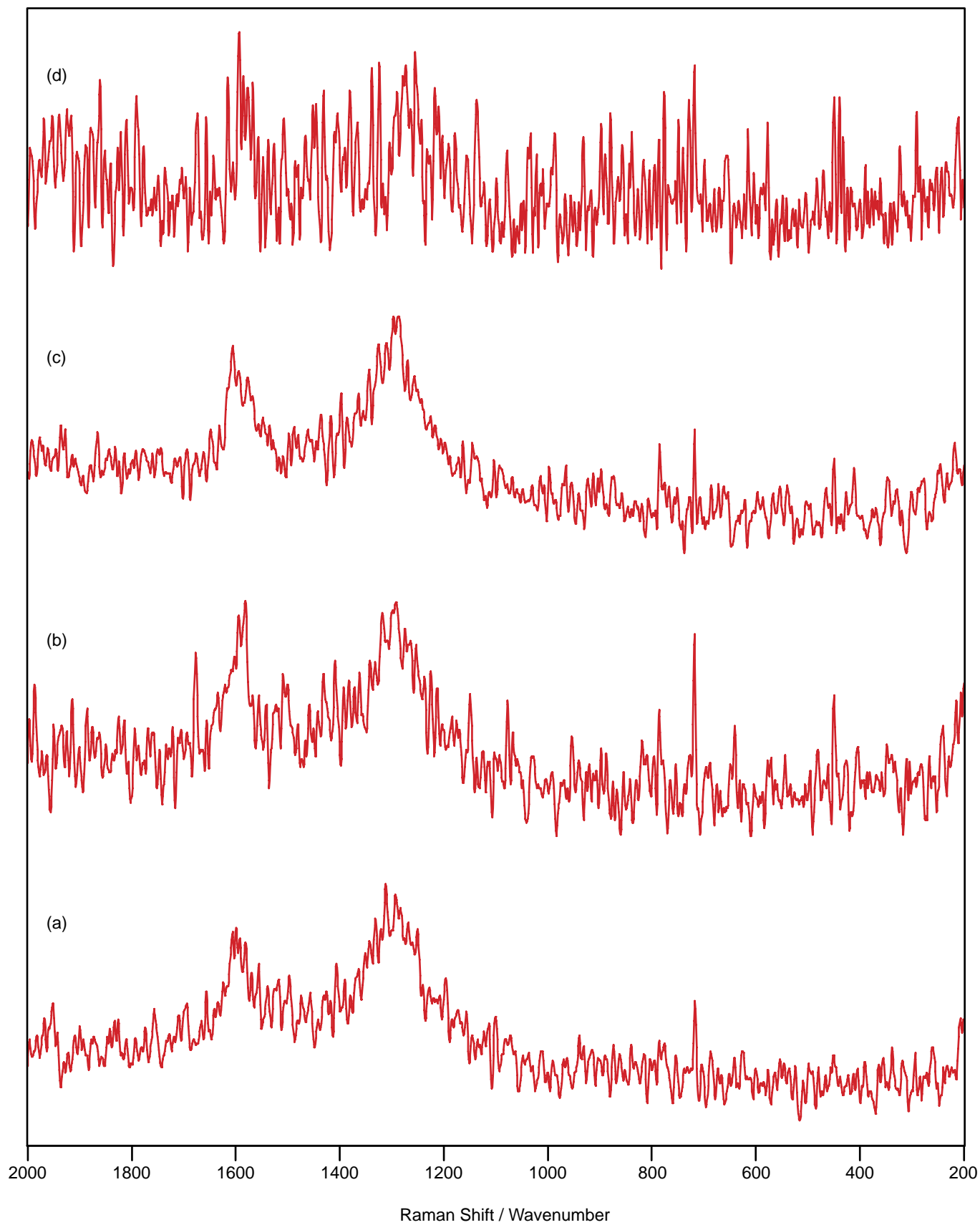
Figure 6: Spectra of graphite: (a) solid, 50mW laser power, 4\text{cm}^{-1} resolution, 500 scans; (b) KBr flats / nujol mull, 125mW laser power, 4\text{cm}^{-1} resolution, 1750 scans; (c) KBr disk, 150mW laser power, 4\text{cm}^{-1} resolution, 1500 scans; (d) KCl disk, 300mW laser power, 4\text{cm}^{-1} resolution, 250 scans.
