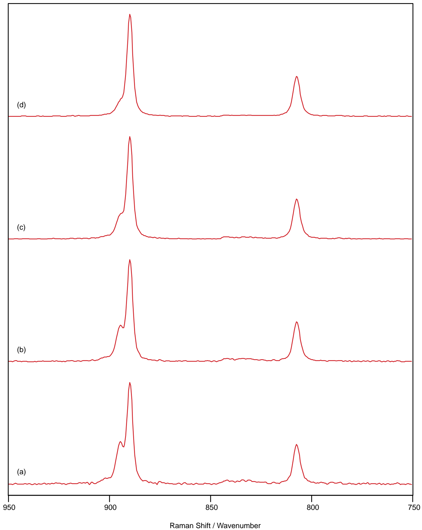
Figure 3: Spectra of \text{Na}_2\text{MoO}_4 recorded at a sample temperature of 70^\circ\text{C} , 1\text{cm}^{-1} resolution and using a laser power of 125\text{mW} for: (a) 10 scans, (b) 20 scans, (c) 40 scans and (d) 70 scans.
