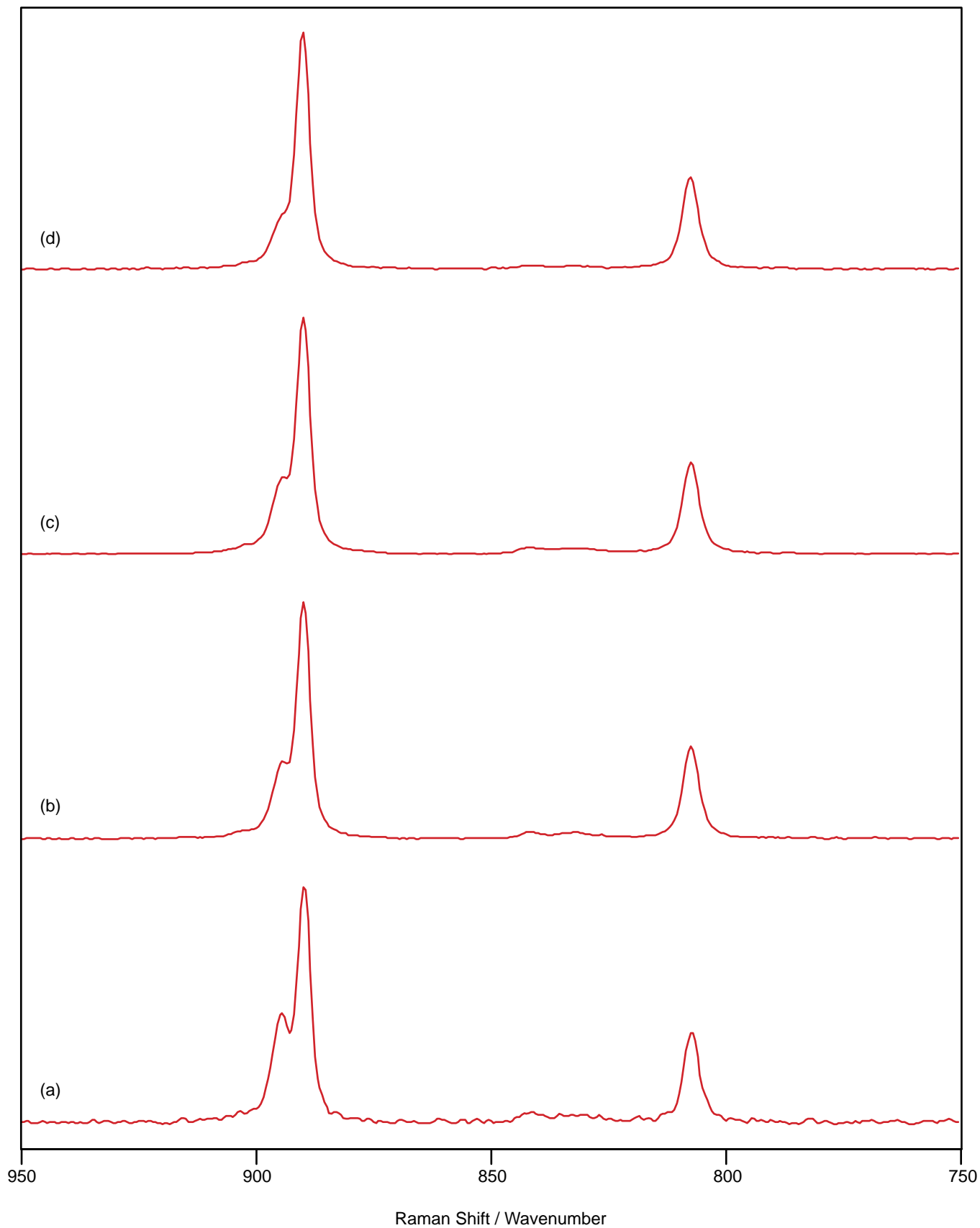
Figure 2: Spectra of \text{Na}_2\text{MoO}_4 recorded for a sample temperature of 70^\circ\text{C} , 1\text{cm}^{-1} resolution, five scans and laser powers of: (a) 125mW, (b) 375mW, (c) 625mW and (d) 875mW
