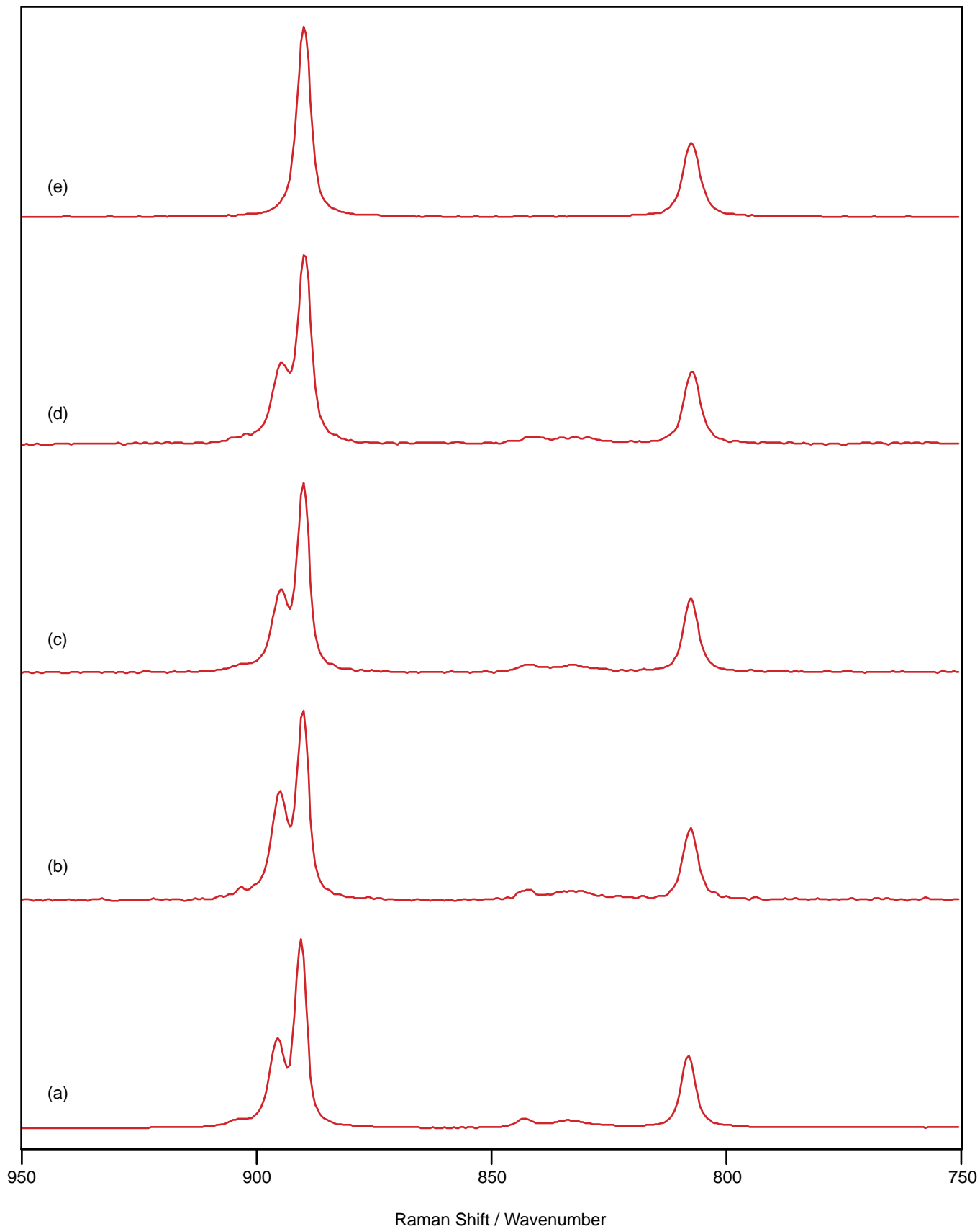
Figure 1: Spectra of Na 2 MoO 4 recorded using a laser power of 250mW, 1cm -1 resolution, five scans and sample temperatures of: (a) 20°C, (b) 40°C, (c) 55°C, (d) 70°C and (e) 80°C.
